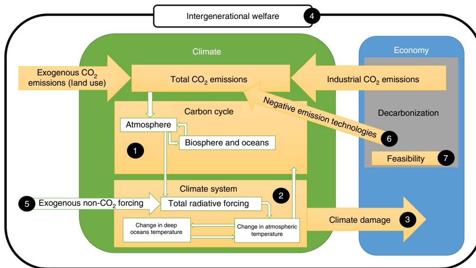
Fig. 1 | Updates to the DICE model. A stylized schematic of the DICE model that highlights the seven updates we make to the standard DICE version (2016R2; ref. 34 ). These are: (1) a carbon cycle based on the FAIR model 29,30 , (2) an update of the EBM 37 , (3) a revised economic damage estimate 28 , (4) a range of expert views on intergenerational welfare 24 , (5) non-CO 2 forcing in line with lower emission pathways 31 , (6) the earlier availability of NETs 2 and (7) constraints on the maximum rate of decarbonization 2,33 .
